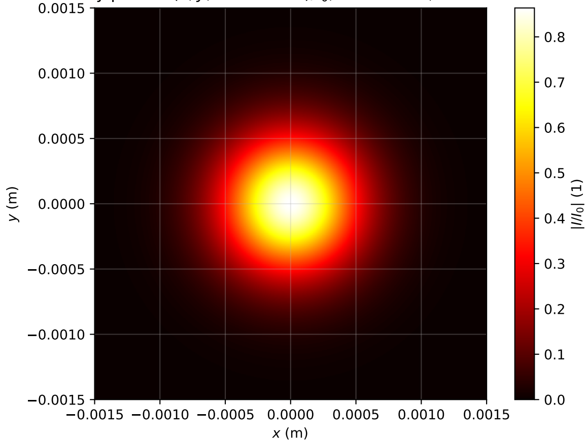
Intensity profile I(x, y, z = 1.274m)/I_0 , Pin=0.3Pcr, artificial time
